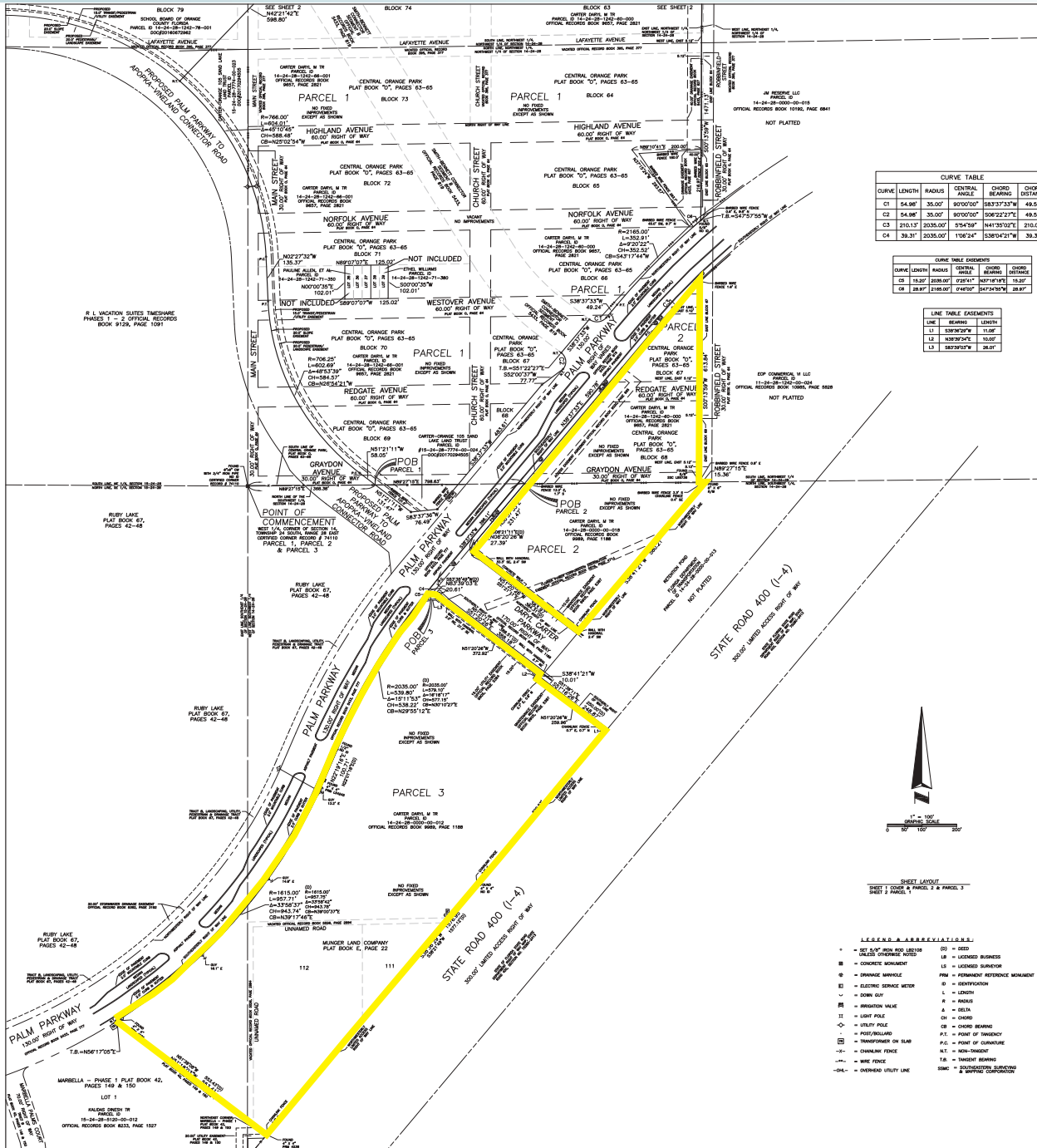
27.3± ACRE TRACT SURVEY
